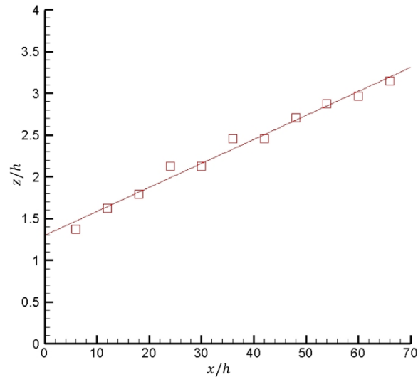
Fig. 11 Critical point in the streamwise x direction
