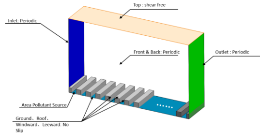
Fig. 2 Boundary conditions
