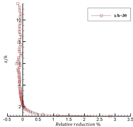
Fig. 9 Relative reduction in diffusion time scale \frac{(\tau_{Pollutant1} - \tau_{NO})}{\tau_{Pollutant1}} \times 100\% . (at x/h = 30 )
