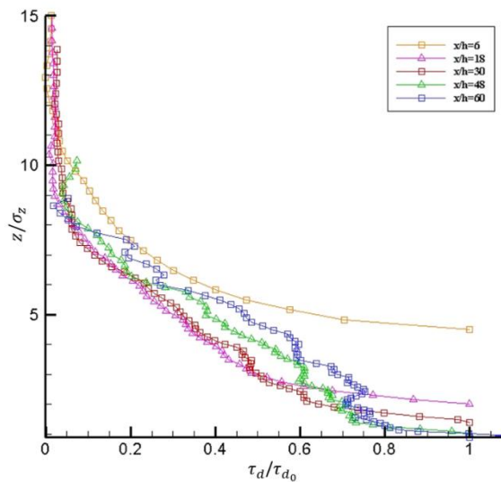
Fig. 4 Diffusion time scale for NO
