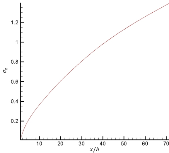
Fig. 3 Dispersion coefficient of NO
