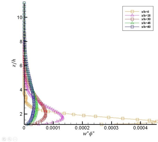
Fig. 5 \langle w''\phi'' \rangle of NO
