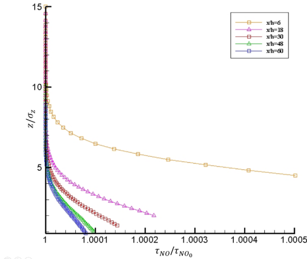
Fig. 7 Reaction time scale of NO
