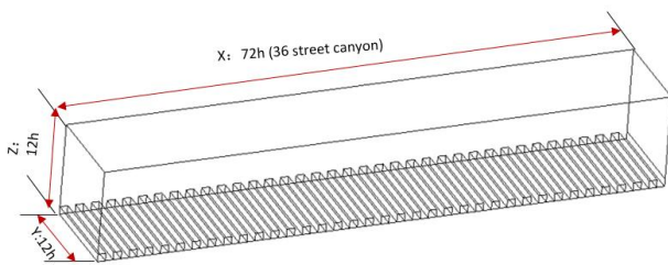
Fig. 1 computational domain
