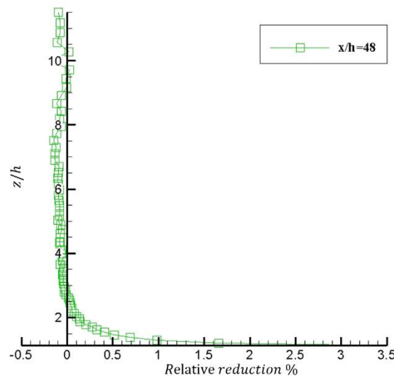
Fig. 10 Relative reduction in diffusion time scale \frac{(\tau_{Pollutant1} - \tau_{NO})}{\tau_{Pollutant1}} \times 100\% . (at x/h = 48 )
