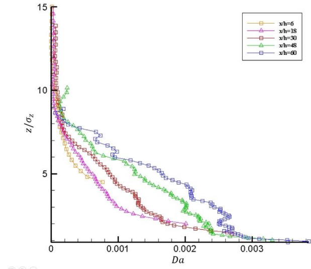
Fig. 8 Damköhler number of NO
