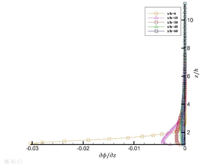
Fig. 6 \partial \langle \bar{\phi} \rangle / \partial z of NO
