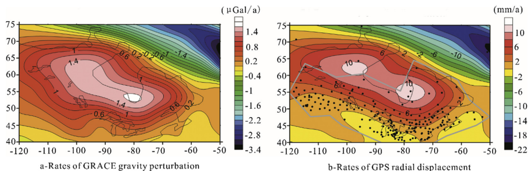
Fig. 1 – GRACE and GPS data used for separating the hydrology signal in North America. a – Trend rates of gravity perturbation from CSR RL05 GRACE monthly data (degree 2 to 60) from August, 2002 to June, 2014; b – Trend rates of radial displacement (degree 2 to 60) derived from the GPS observations from 1993 to 2006 [15]. Thick light gray line surrounds the investigation area which depends on a dense GPS network. The black dots denote the GPS sites.
