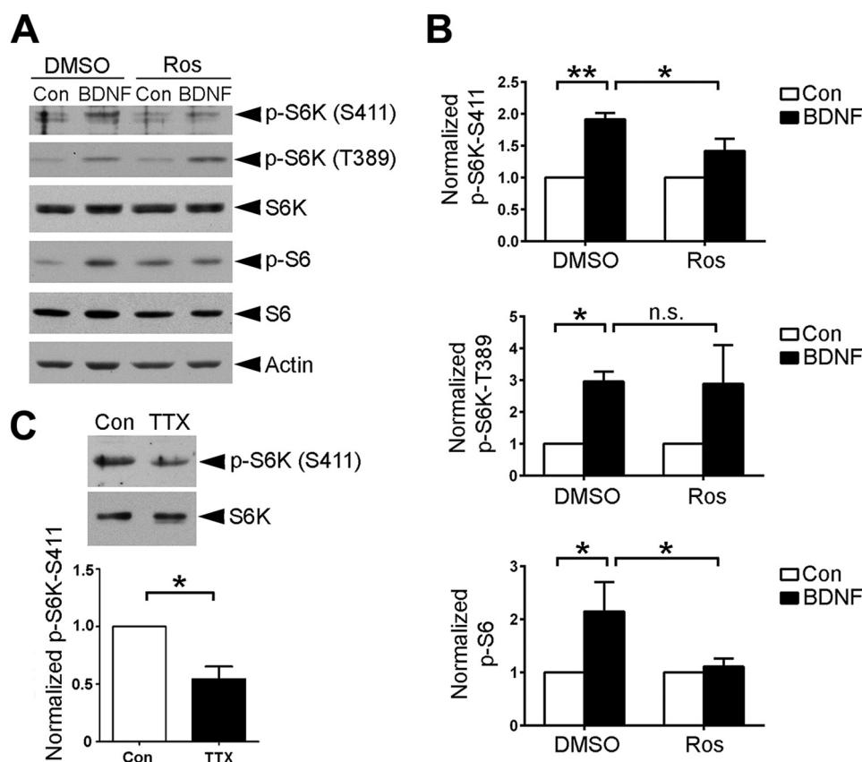
FIGURE 4. Regulation of S6K Ser-411 phosphorylation by BDNF and neuronal activity. A, S6K phosphorylation at Ser-411 was induced by BDNF in cortical neurons, and the induction of S6K Ser-411 phosphorylation and S6 ribosomal protein phosphorylation was attenuated by roscovitine (Ros). Roscovitine did not affect the induced S6K phosphorylation at Thr-389. B, quantification of the Western blots. The intensity of phospho-S6K and phospho-S6 was normalized with total S6K and total S6, respectively. Three independent experiments were performed (*, p < 0.05 ; **, p < 0.01 ; one-way ANOVA, Tukey's or Bonferroni's multiple comparison tests; error bars represent S.E.). C, treatment of cortical neurons (14–17 DIV) with TTX (2 μM for 24 h) significantly reduced Ser-411 phosphorylation of S6K (three independent experiments were performed; *, p < 0.05 ; n.s., not significant; Student's t test; error bars represent S.E.). Con, control.
