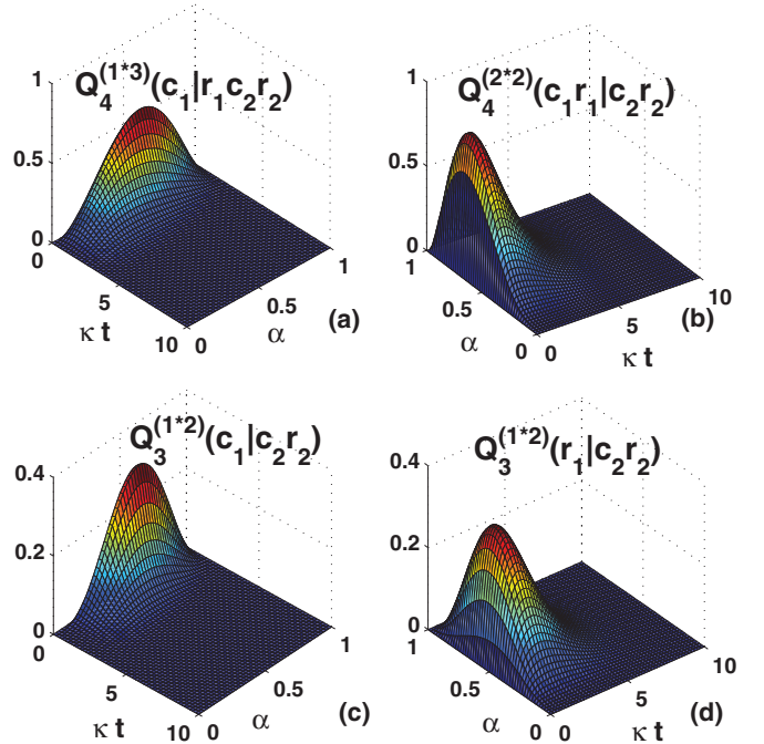
FIG. 4. (Color online) Different components of multipartite quantum correlation indicators in cavity-reservoir systems as a function of the time evolution \kappa t and the initial state amplitude \alpha , where all the correlation distributions are non-negative and detect the genuine multipartite quantum correlations.
