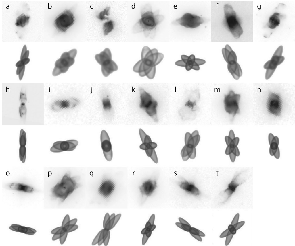
Figure 3. Comparison of the 20 observed images (those with an index letter) with its corresponding modeled image (the one right below it). Brightness levels are in log scale. North is pointing up and east to the left. Refer to Table 1 for the object data. The angular sizes and brightness levels of the objects are not the same.
