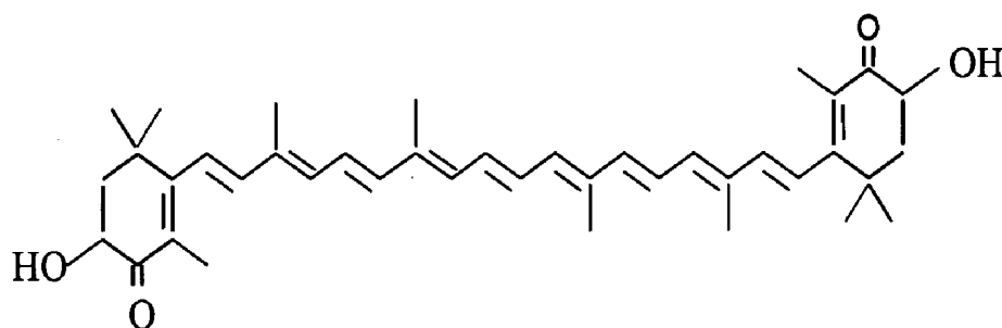
Astaxanthin
