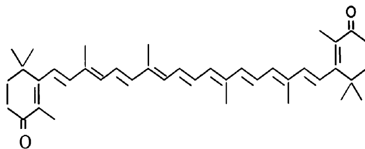
Canthaxanthin
