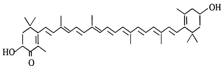
Adonixanthin
