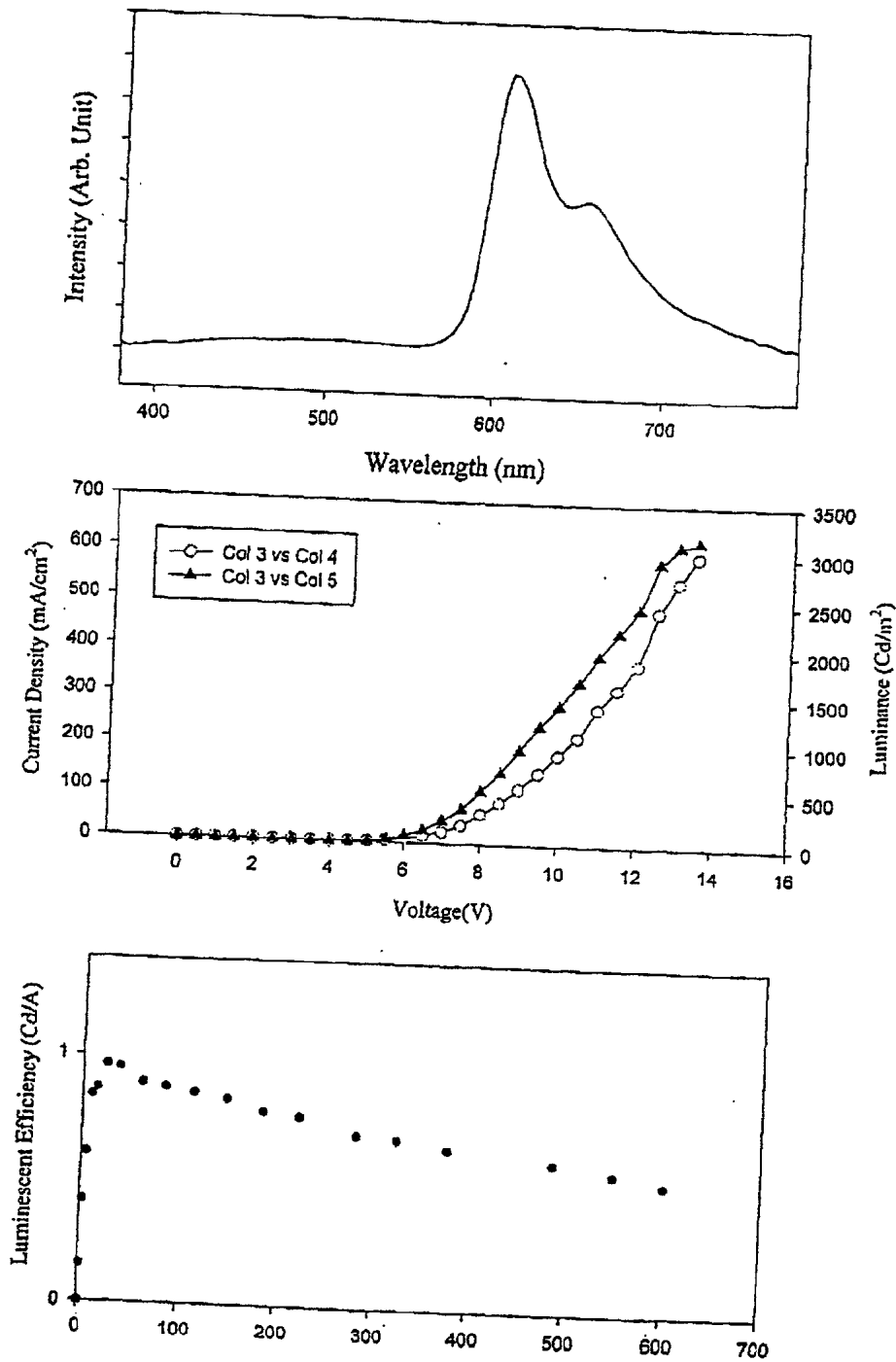
Figure 10. Electroluminescent spectrum, current-voltage (I-V) and luminance-voltage (B-V) curves and luminescent efficiency-current density curve of the device using complex 16 as emitter with a doping level of 4%.
