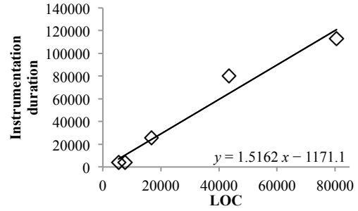
Figure 12. Effect of program length on instrumentation duration.
