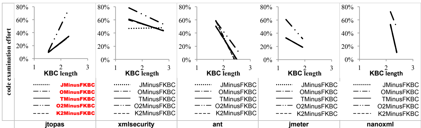
Figure 10. Impacts of KBC length on fault localization effectiveness for different programs.
