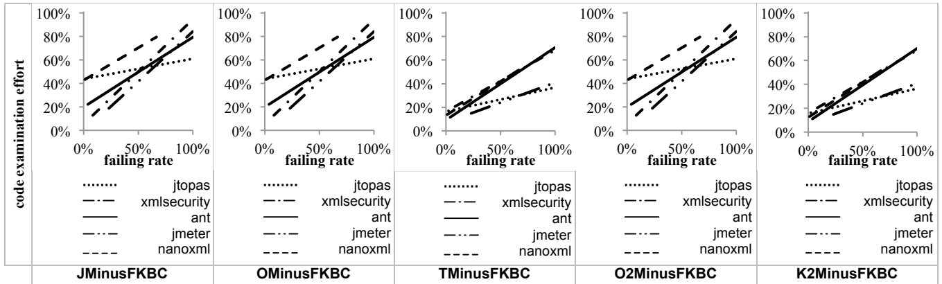
Figure 7. Impacts of failing rate on fault localization effectiveness for different techniques.
