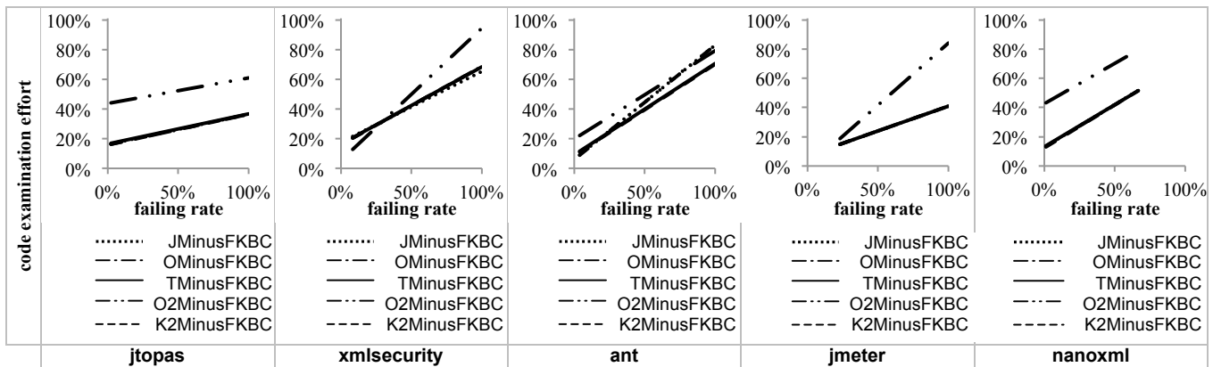
Figure 8. Impacts of failing rate on fault localization effectiveness for different programs.
