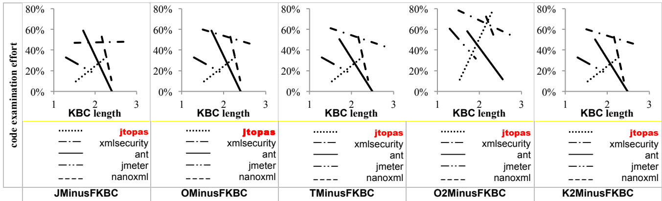
Figure 9. Impacts of KBC length on fault localization effectiveness using different techniques.
