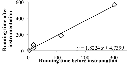
Figure 11. Correlation of program running times before and after instrumentation.
