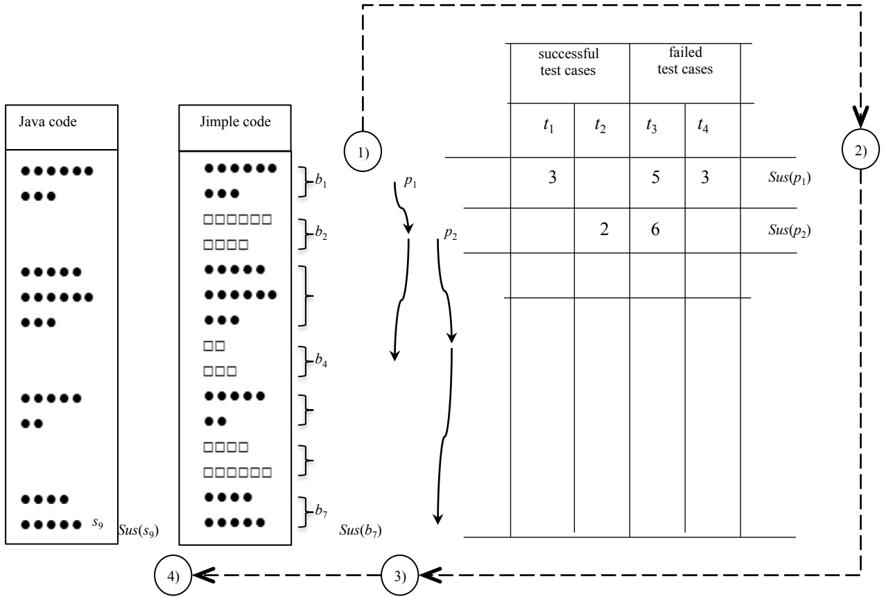
Figure 4. Overview of our framework.
