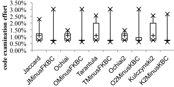
Figure 13. Result on the 2-fault versions of jtopas 0.4.
