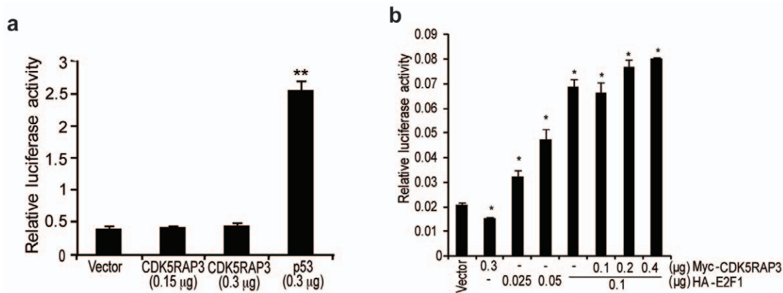
Figure 4. CDK5RAP3 transcriptionally regulated p14 ARF in a E2F1 independent manner. (a) CDK5RAP3 was co-transfected with p53-responsive element reporter for luciferase assay in HepG2 cells. Results represent mean \pm SD for triplicate wells. *, P < 0.05 , **, P < 0.005 compared with vector control, Student's t -test. (b) Expression constructs of CDK5RAP3 was co-transfected with HA-E2F1 and p14 ARF -luc reporter for luciferase assay in HepG2 cells. Results represent mean \pm SD for triplicate wells. *, P < 0.005 compared with vector control, Student's t -test. doi:10.1371/journal.pone.0042210.g004
