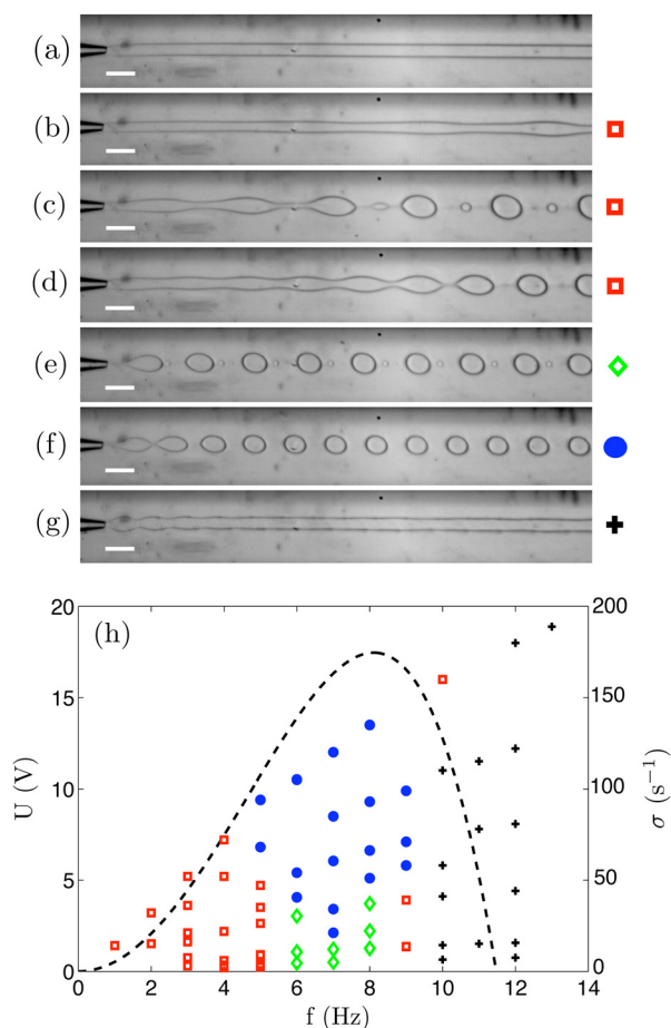
FIG. 2. Different flow regimes as a function of the frequency of the forcing. The inner and outer fluid flow rates are, respectively, Q_{in} = 50 \mu\text{l h}^{-1} and Q_{out} = 5000 \mu\text{l h}^{-1} . Optical image of the jets and drops observed (a) in the absence of external forcing, f = 0 Hz, (b) at f = 3 Hz, (c) f = 4 Hz, (d) f = 6 Hz, (e) f = 7 Hz, (f) f = 8 Hz, and (g) f = 10 Hz (scale bars are 200 \mu\text{m} ) (see Ref. 20). A state diagram of the different regimes as a function of the frequency of the forcing (in Hz) and the input voltage applied to the mechanical vibrator (in volts, left scale) is represented in (h). The dashed-dotted line is the growth rate of the Rayleigh-Plateau instability (right scale) (see Ref. 22) (enhanced online) [URL: http://dx.doi.org/10.1063/1.3702434.1 ] [URL: http://dx.doi.org/10.1063/1.3702434.2 ] [URL: http://dx.doi.org/10.1063/1.3702434.3 ] [URL: http://dx.doi.org/10.1063/1.3702434.4 ] [URL: http://dx.doi.org/10.1063/1.3702434.5 ] [URL: http://dx.doi.org/10.1063/1.3702434.6 ] [URL: http://dx.doi.org/10.1063/1.3702434.7 ] [URL: http://dx.doi.org/10.1063/1.3702434.8 ].
