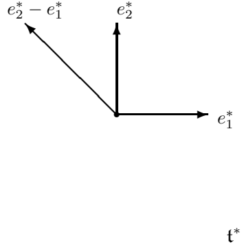
(a) An example of isotropy weights at a fixed point p \in F when \dim T = 2 , \dim_{\mathbb{C}} M = 3 .
