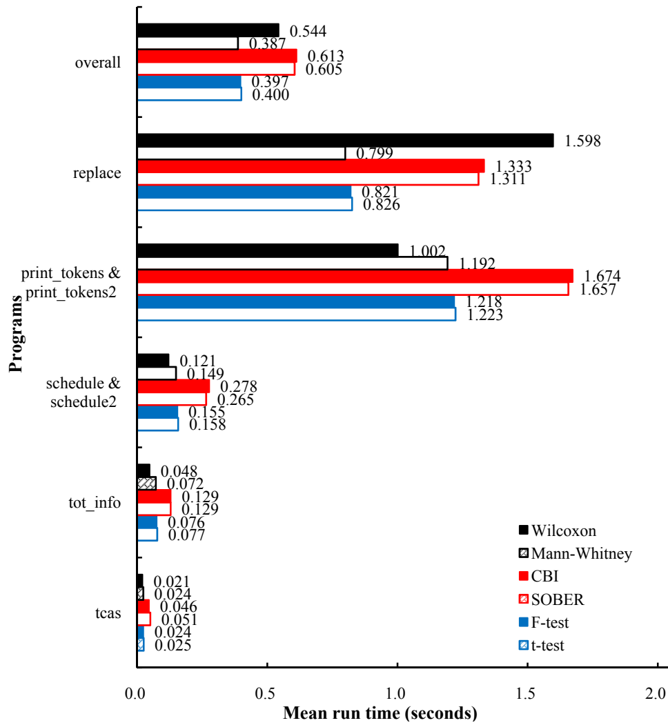
Figure 12: Time spent by each technique on subject programs.
