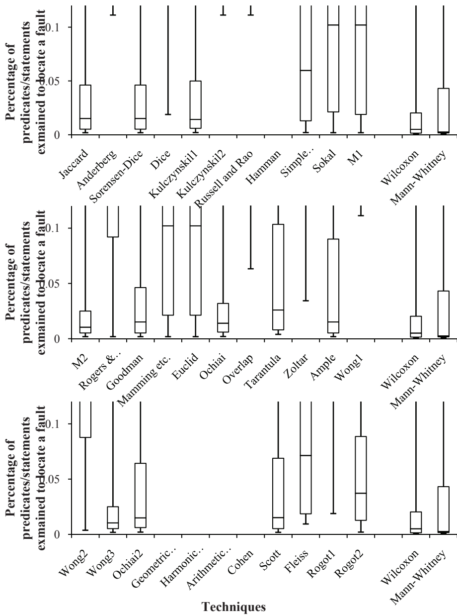
Figure 9: Effectiveness comparison between non-parametric methods and statement-level techniques (zoomed in).
