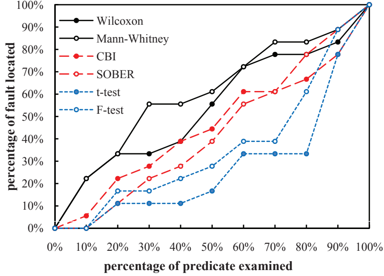
Figure 3: Individual effectiveness comparison on schedule and schedule2.
