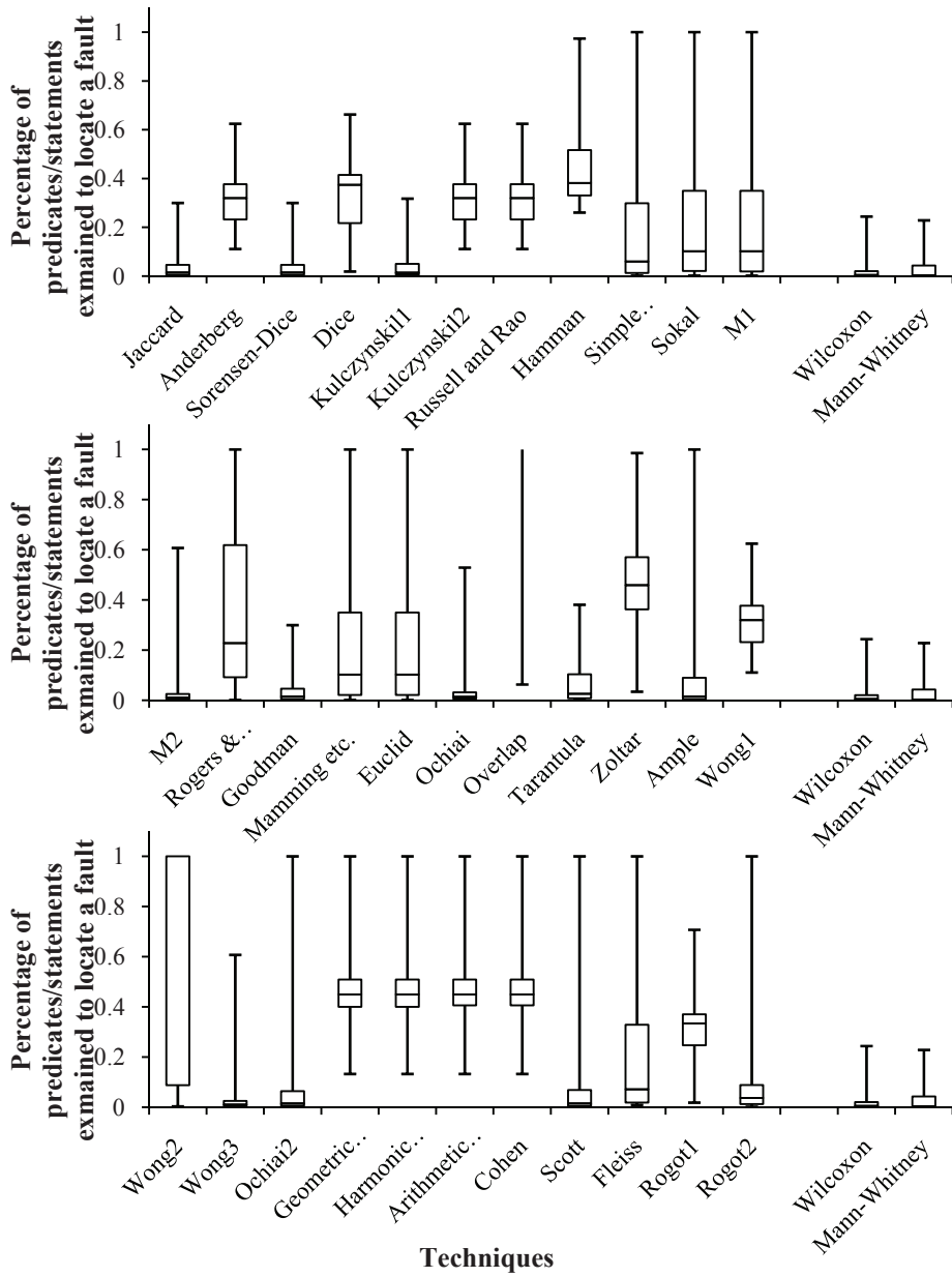
Figure 8: Effectiveness comparison between non-parametric methods and statement-level techniques.
