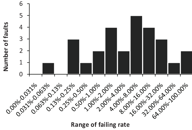
Figure 7: Histogram for failing rate distribution of the 28 faulty versions of space.
