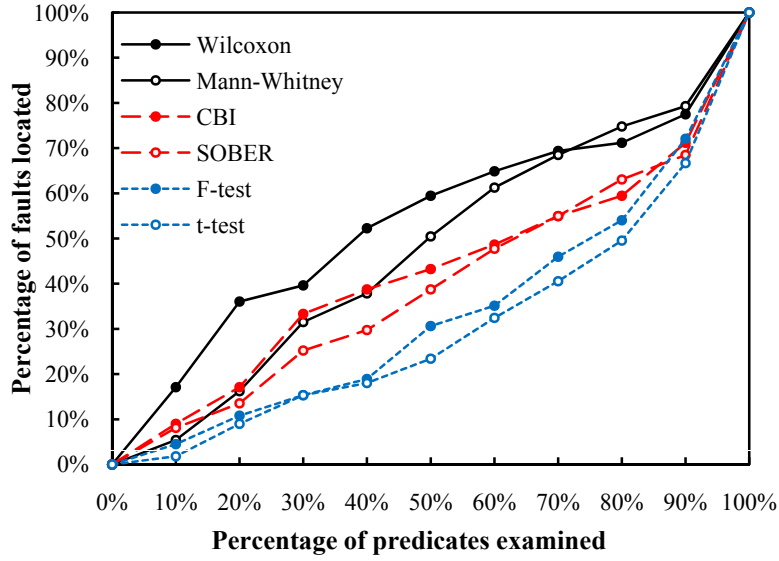
Figure 1: Overall effectiveness comparison.
