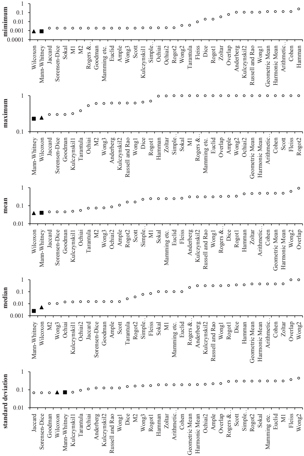
Figure 10: Minimum, maximum, mean, median, and standard deviation of effectiveness of TC3 and TC4 techniques over the space program.
