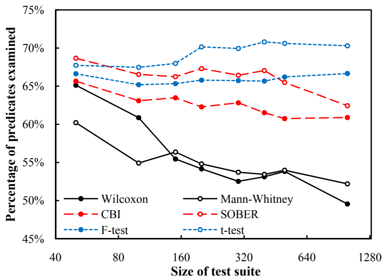
Figure 11: Effect of test suite size. (The lower the curve is, the better will be the technique.)
