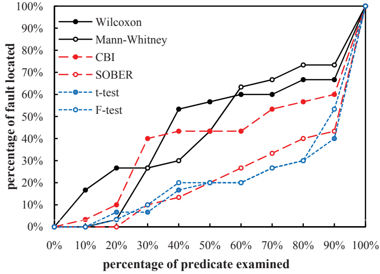
Figure 4: Individual effectiveness comparison on tcas.
