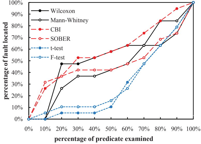
Figure 5: Individual effectiveness comparison on tot_info.
