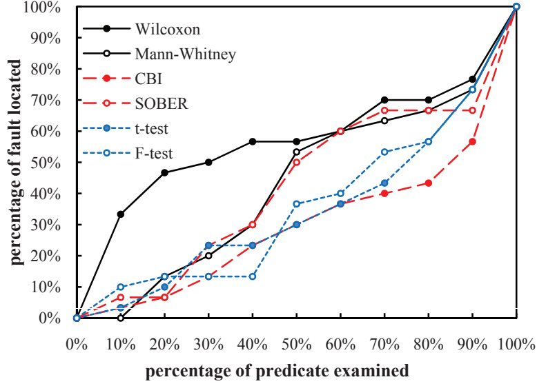
Figure 2: Individual effectiveness comparison on replace.
