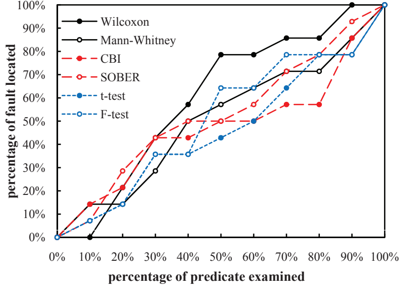
Figure 6: Individual effectiveness comparison on print_tokens and print_tokens2.
