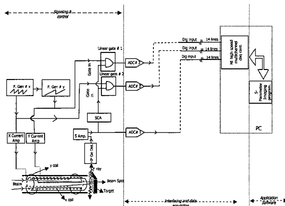
Block diagram of the complete imager setup circuitry applied to positron beam.
