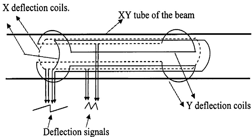
Fig 5 : Side view of the XY deflection coils.
