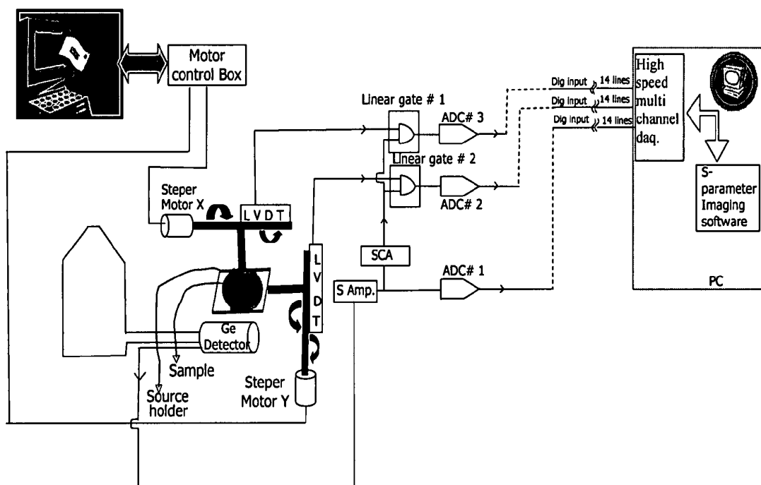
Fig12 : Complete scheme of the basic imager.
