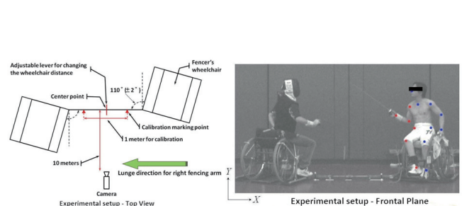
Figure 4. Experimental setup
