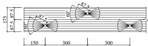
Figure 2. FRP strengthening scheme for Slabs S2 and S7 and anchor layout for Slab 7
