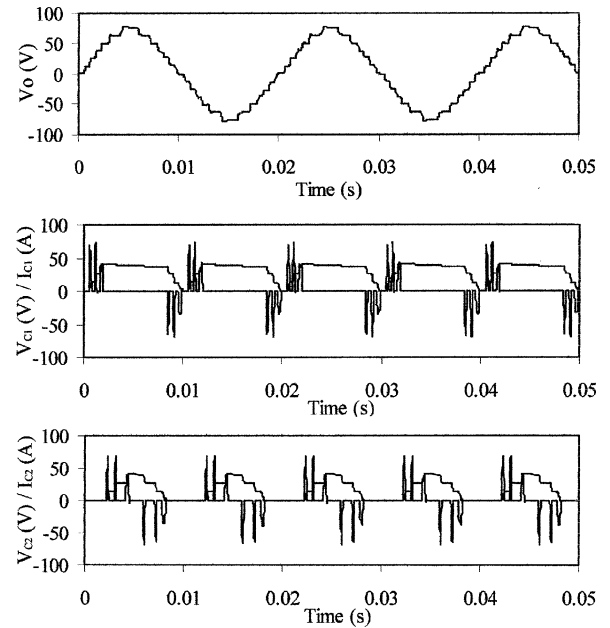
Fig. 5. PSPICE-simulated waveforms.
