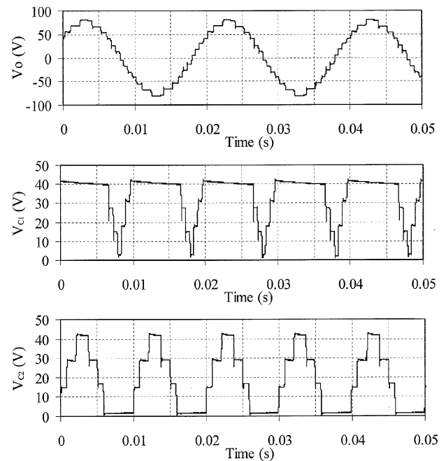
Fig. 6. Measured waveforms.
