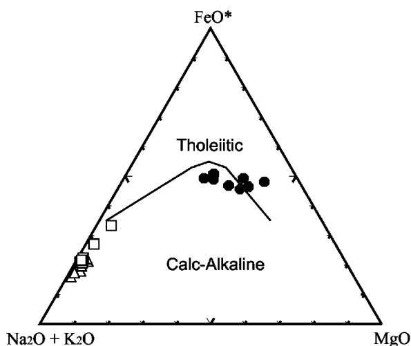
Figure 5. AFM ( [\text{Na}_2\text{O} + \text{K}_2\text{O}] - \text{FeO}^* - \text{MgO} ) plot of the Baiyin volcanic rocks, NW China (reference fields after Irvine and Baragar 1971). Symbols are the same as those for figure 4.
