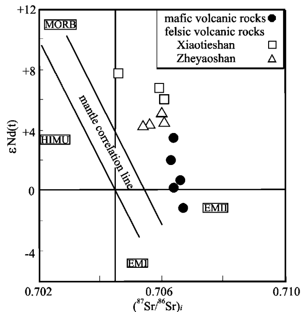
Figure 8. Initial Sr-Nd isotopic compositions of the Baiyin volcanic rocks, NW China.
