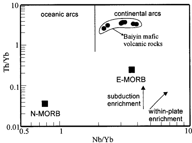
Figure 9. Plot of Nb/Yb versus Th/Yb for the Baiyin mafic volcanic rocks, NW China (reference fields are after Dunphy and Ludden 1998). Normal mid-ocean ridge basalt ( N-MORB ) and enriched mid-ocean ridge basalt ( E-MORB ) values after Sun and McDonough (1989).
