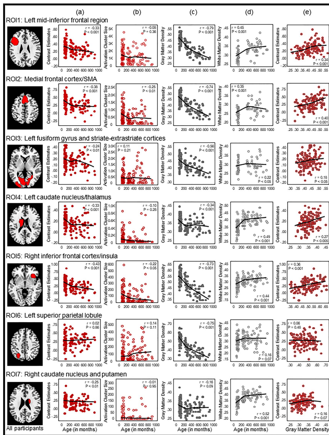
Figure 3. ROI-based Pearson correlation analyses. Seven ROIs surviving the stringent voxel-level P < 0.001 FWE threshold in the all-participant homophone > font activation map were selected. Pearson correlations between age and (a) BOLD signal activity, (b) activation cluster size, (c) GM density, and (d) WM density at each of the seven ROIs are shown in columns (a)–(d), respectively. Columns (e) and (f) respectively show Pearson correlations of BOLD signal activity with GM density and WM density. Pearson correlations between Chinese character reading performance and BOLD signal activity, activation cluster size, GM density and WM are shown, respectively, in columns (h) to (j). In each scatterplot, a fit line was added by using a local regression (LOESS) method (Epanechnikov kernel, 80% of points to fit, 95% confidence intervals).
