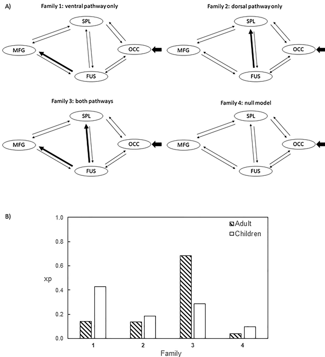
Figure 5. (A) Families of DCM models. The short arrows pointing at OCC represent the input of the effects of the experimental condition (homophone judgment). Thick arrows in families 1–3 represent the presence of the modulatory effects of the experimental condition. Apart from the two connections designated for family partition, all the other connections are allowed to be switched on and off for modulatory effects. This results in 2^8 = 256 models in each family. (B) The xp of each family in the adult and children group.
