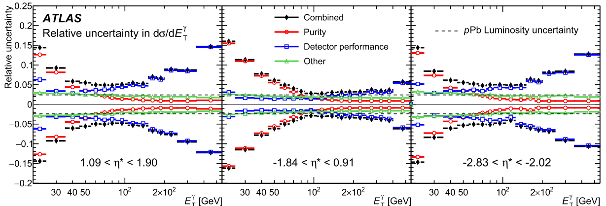
Fig. 4. Summary of the relative sizes of major sources of systematic uncertainty in the cross-section measurement, as well as the combined uncertainty (excluding luminosity), shown as a function of photon transverse energy E_T^{\gamma} .
