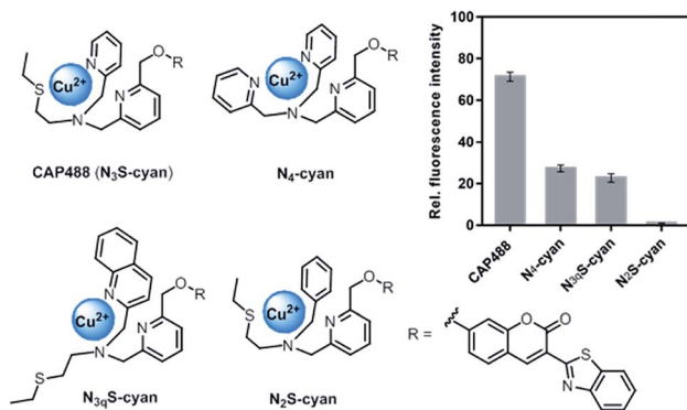
Fig. 1 Structures and fluorescence response towards 1 eq. of dopamine of \text{Cu}(\text{II}) complex–fluorophore conjugates with combinations of N,S-donors.
