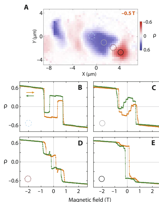
Fig. 4. Position-sensitive ferromagnetic domain dynamics. (A) Spatial map of \rho from Fig. 3 ( -0.5\text{ T} , sweep down) with blue, gray, brown, and black circles indicating the spots of selected magnetic field sweeps of \rho in (B), (C), (D), and (E).
