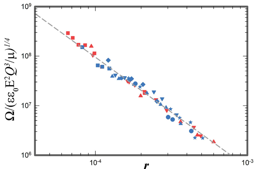
Figure 2. A log-log plot of \Omega / (\epsilon\epsilon_0 E^2 Q^3 / \mu)^{1/4} against jet radius, r , based on the scaling law (1). The red and blue symbols correspond to different viscous liquids, lecithin from soy bean and polyglycerolpolyricinoleate (PGPR), respectively. The shape of symbols corresponds to different flow rates of 10 ml/h (■), 20 ml/h (◆), 30 ml/h (▼), 50 ml/h (▲), 70 ml/h (●), 150 ml/h (★), respectively. The size of the nozzle used for flow rates of 10 ml/h, 20 ml/h, 30 ml/h and 50 ml/h is 0.92 mm, and that for flow rates of 70 ml/h and 150 ml/h is 1.4 mm. All data are fitted by the relation \Omega / (\epsilon\epsilon_0 E^2 Q^3 / \mu)^{1/4} \sim r^{-9/4} , represented by the grey dash line, confirming the scaling law (1).
