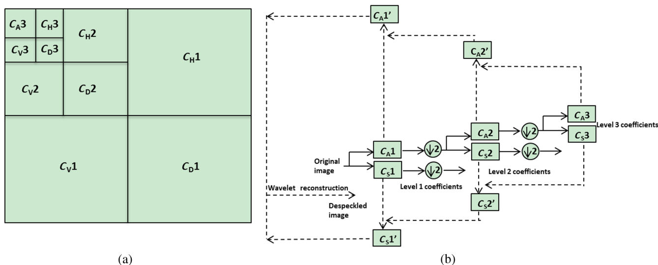
Fig. 1 (a) Ordering of the approximation and detailed coefficients of a three-level two-dimensional discrete wavelet transform (2-D-DWT) and (b) step-by-step flowchart of the proposed method (three-level DWT). Solid arrows represent 2-D-DWT. Dashed arrows represent the procedure for compounding process and 2-D-IDWT.
