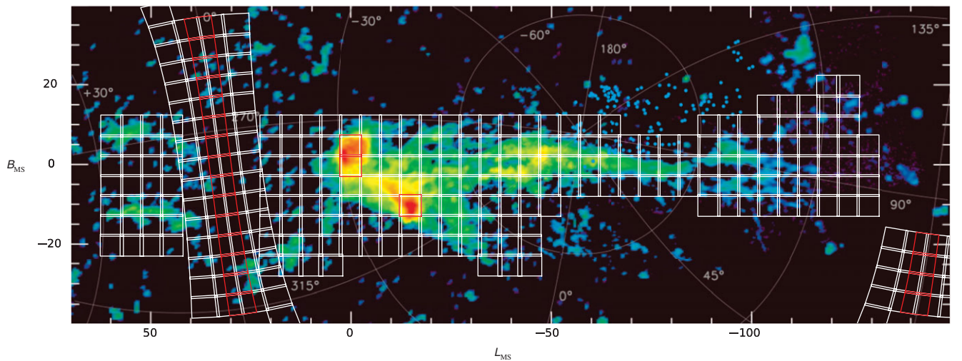
Figure 3. The GASKAP MS survey area with axes labeled in MS coordinates and H I column densities from the LAB survey in the background (Nidever et al. 2010). The white squares represent ASKAP pointings with the shorter integration time (12.5 h), while the red squares are pointings that will be observed for either 50 or 200 h.
