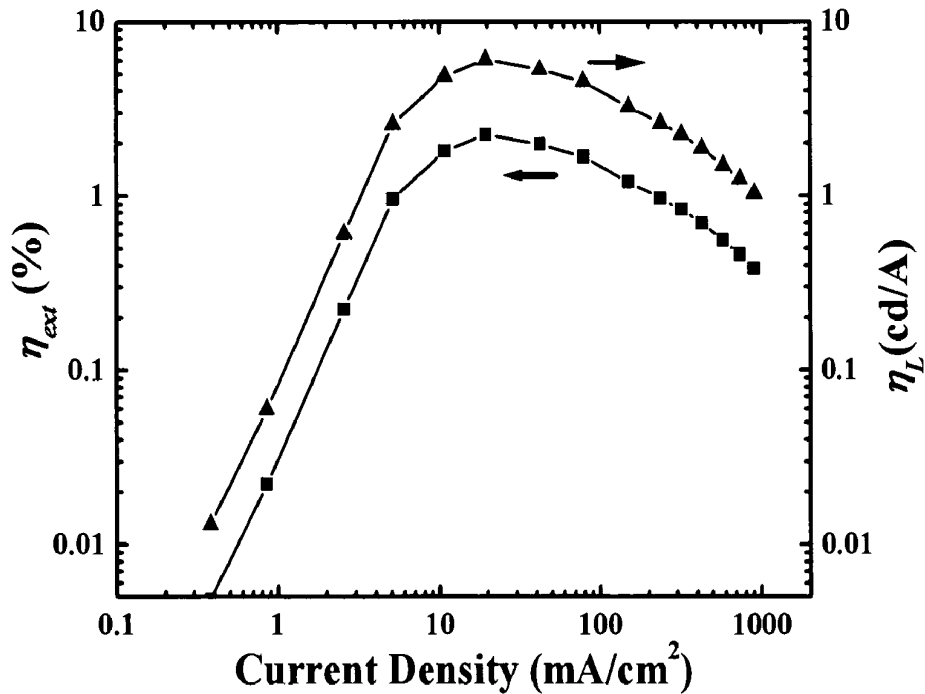
FIG 16. The external quantum efficiency and luminous efficiency of OLED C with 3.0 wt.% dopant 19
