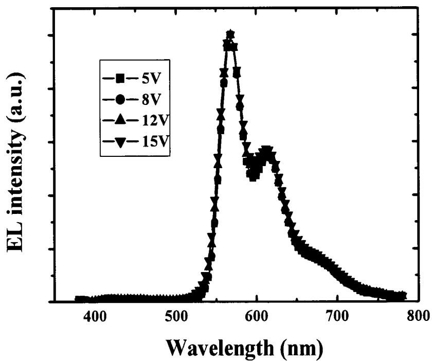
FIG 10. EL spectra of OLED B with 5 wt.% dopant 3 at different applied voltages
