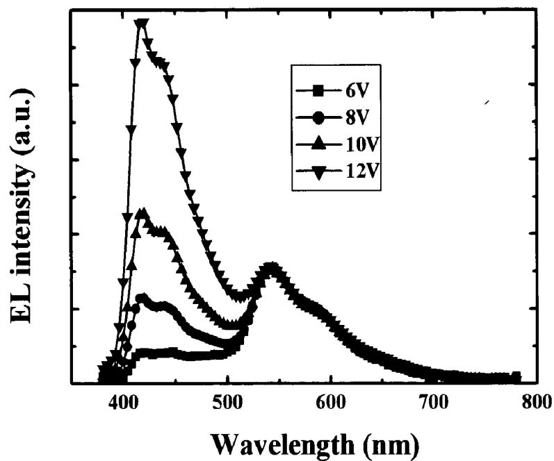
FIG 18. EL spectra of OLED D with 4 wt.% dopant 51 at different applied voltages
