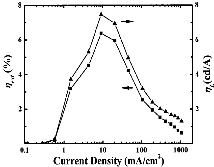
FIG. 28 External quantum efficiency and luminous efficiency of OLED F with 1.6 wt.% dopant 104
