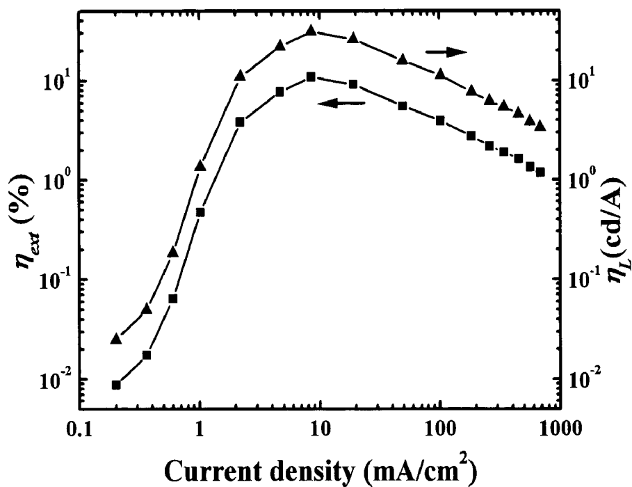
FIG 20. The external quantum efficiency and luminous efficiency of OLED D with 4.0 wt.% dopant 51
