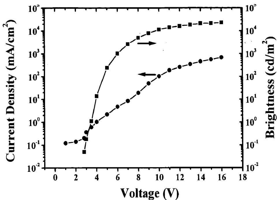
FIG 19. V-I-B curve of OLED D with 4 wt.% dopant 51
