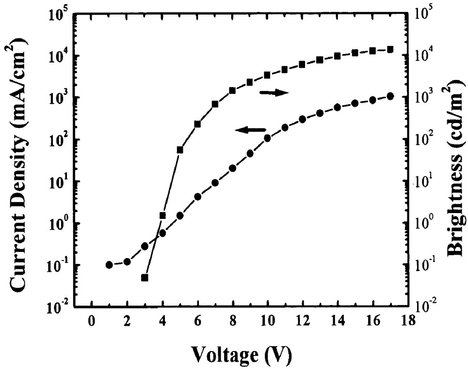
FIG. 27 V-I-B curve of OLED F with 1.6 wt.% dopant 104
