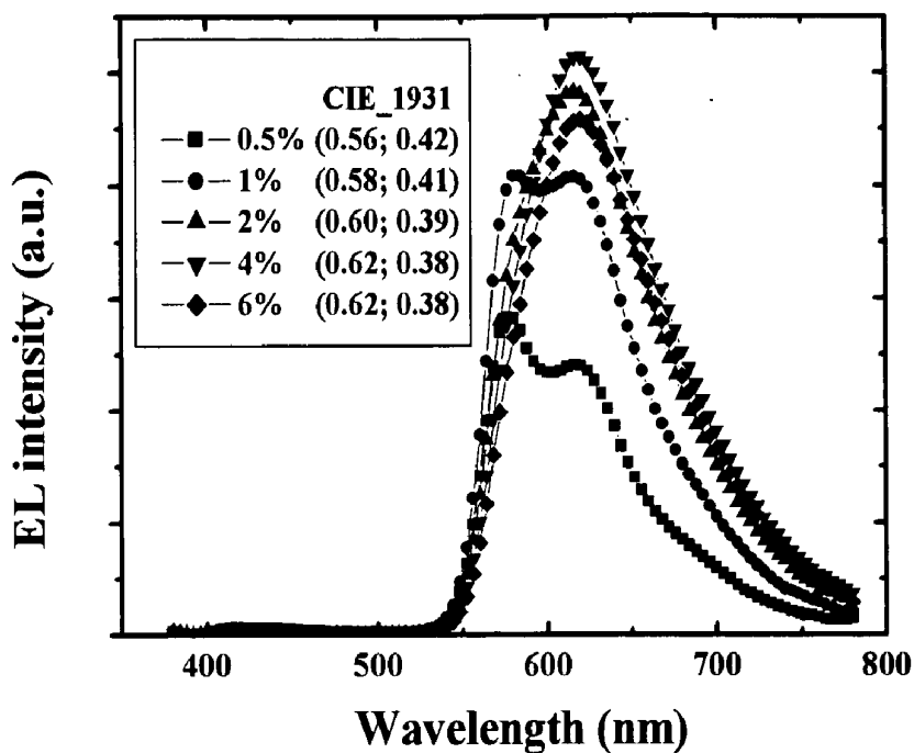
FIG 5. EL spectra of OLED A with 4.0 wt.% dopant 1 at different dopant concentrations under 8 V
