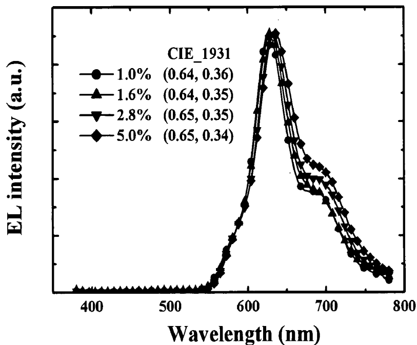
FIG. 25 EL spectra of OLED F with 1.6 wt.% dopant 104 at different dopant concentrations at 8 V
