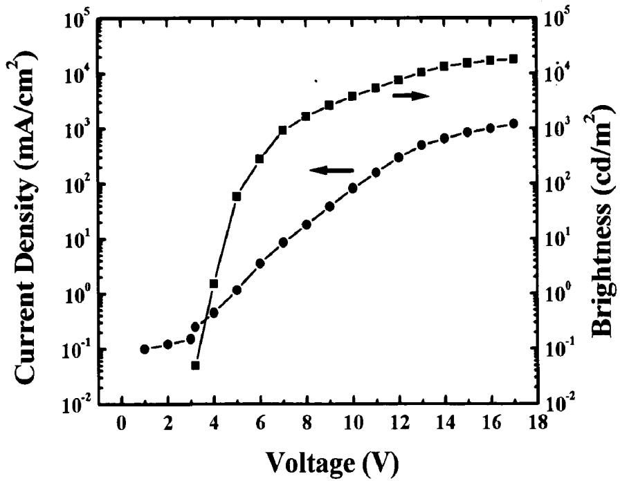
FIG. 23 V-I-B curve of OLED E with 1.5 wt.% dopant 99
