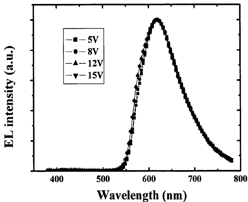
FIG 6. EL spectra of OLED A with 4.0 wt.% dopant 1 at different applied voltages
