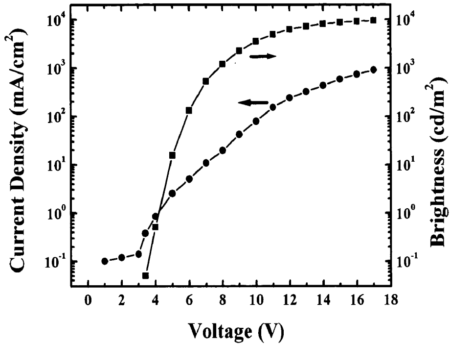
FIG 15. V-I-B curve of OLED C with 3 wt.% dopant 19
