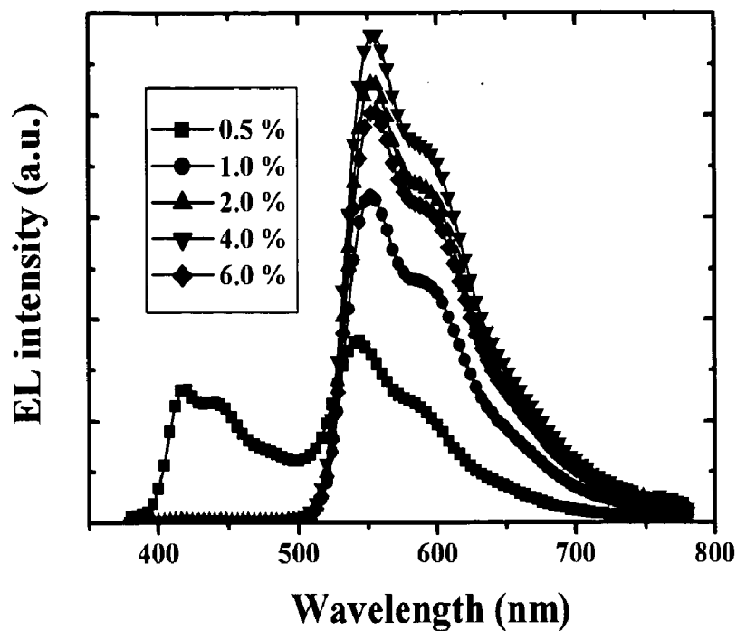
FIG 17. EL spectra of OLED D with 4 wt.% dopant 51 at different dopant concentrations at 8 V
