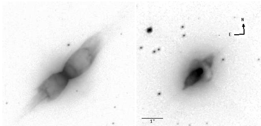
Fig. 6. Left: He2-320 is an example of PNe with highly collimated lobes. Right: A disk can clearly be seen in scattered light in the PPN IRAS 17106–3046 [8].
