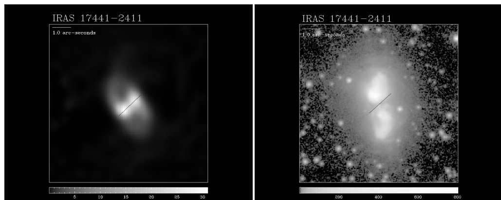
Fig. 3. Gemini T-ReCS 11.7 \mu\text{m} images of PPN IRAS 17441–2411 (left). The orientation of the infrared disk is overlaid on the optical I band HST image (right) as a solid line [21].
