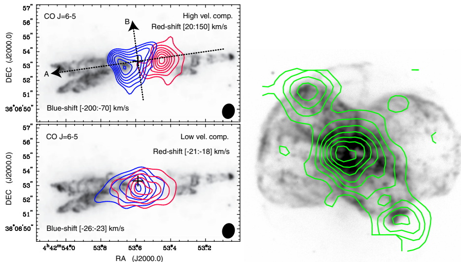
Fig. 2. Left: SMA CO J = 6 - 5 (shown in contours) high- (top panel) and low- (bottom panel) velocity components emission superimposed on the HST H\alpha image of AFGL 618 [13]. Right: CO J = 3 - 2 emission (shown in contours) in NGC 2440 observed with the JCMT overlaid on a [N II] image taken at the CFHT [20].
